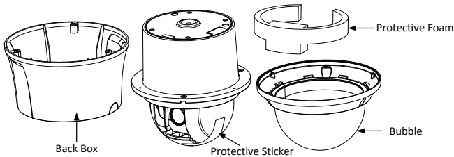
Figure 2-8 Disassemble the Speed Dome
