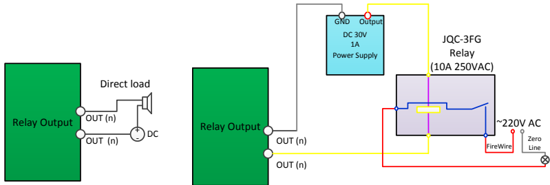
Figure 1-8 Alarm Output
